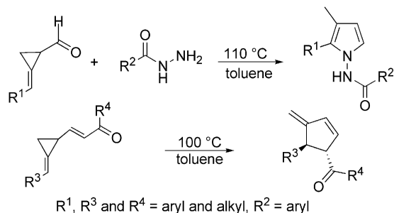
Scheme 1. Previous studies on the ring-opening reactions of MCP derivatives.
