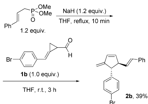
Scheme 2. Tandem Horner–Wadsworth–Emmons olefination/Cope rearrangement of MCP aldehyde 1b with dimethyl cinnamylphosphonate.
