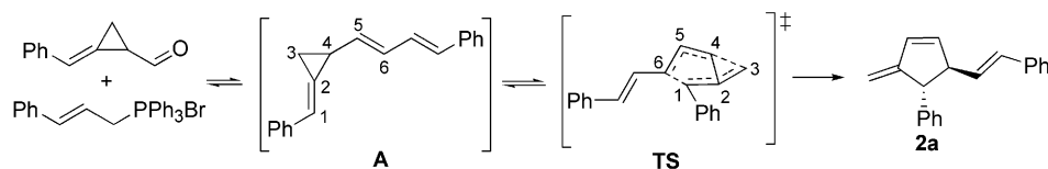
Scheme 4. A plausible reaction mechanism.
