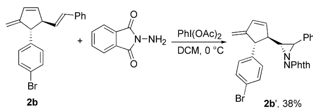
Scheme 3. Azacyclopropanation of 2b .
