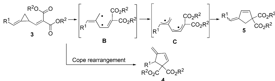
Scheme 5. A plausible reaction mechanism.
